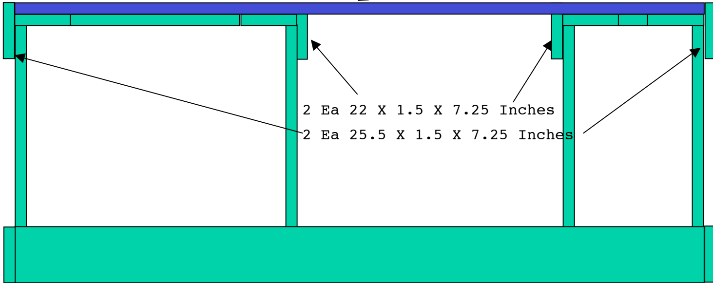
Front View with larger area on left side
