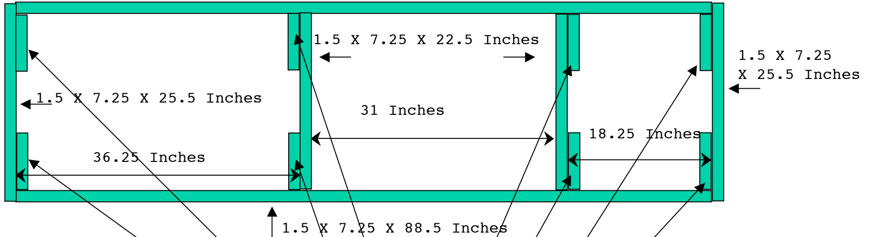
Top View of Bottom Frame
