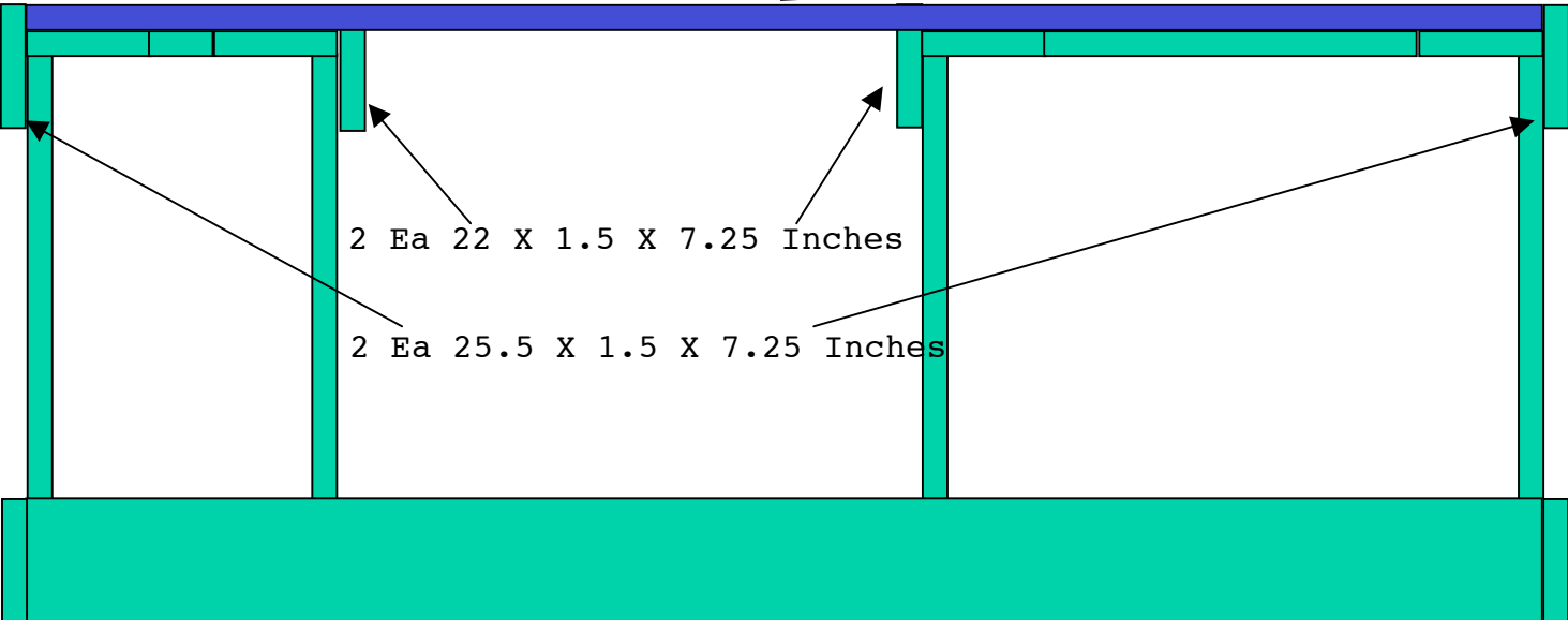
Front View with larger area on Right side
